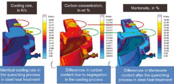
Figure 17. Effect of carbon segregation on martensite formation during quenching.
