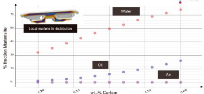
Figure 21. Influence of the carbon content and quench medium on the fraction of martensite in the casting.
