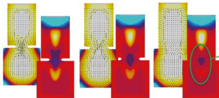
Figure 12 : Predicting under-riser segregation considering feeding and convective flows.
