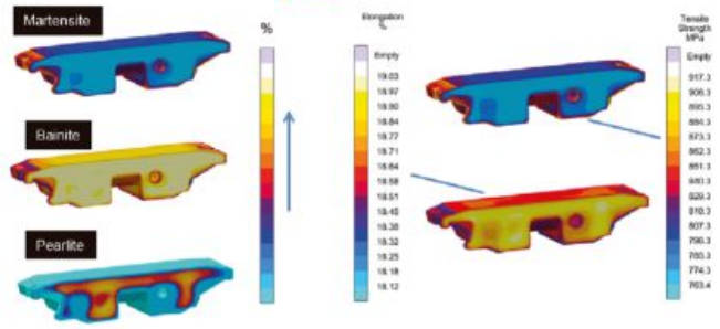
Figure 19. Typical results of the heat treatment simulation of a low alloy steel chain link: predicted microstructures in the cross section after quenching and related mechanical properties.
