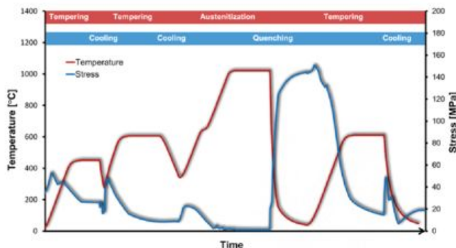
Figure 23. Temperature profile during heat treatment and the corresponding stress development in the interior of the thick section of a blade for a Francis turbine.
