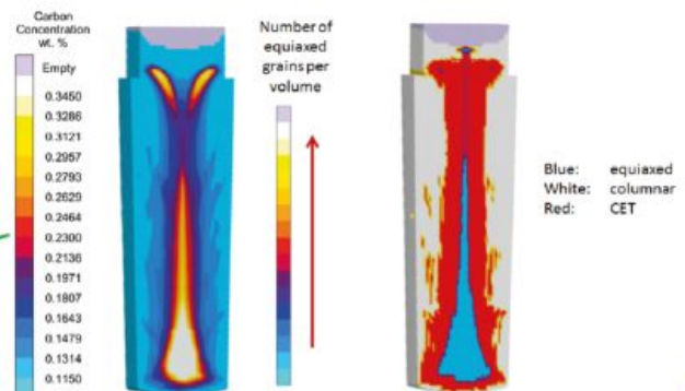
Figure 13 : Predicting grain size and columnar to equiaxed transition in ingot castings.
