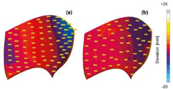
Figure 24. Deviation between the simulated distortion and the target geometry: a) initial calculation and b) after pre-shaping the pattern.
