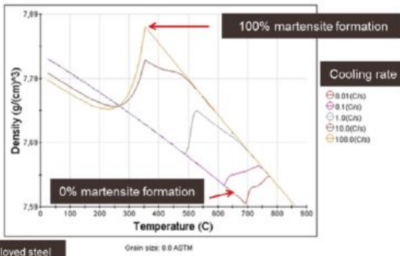
Figure 18. Density as a function of temperature. The density curve changes locally depending on the microstructure formation.
