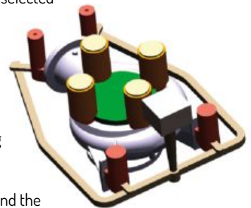
Figure 14. Casting design for a carbon steel pump casing.
