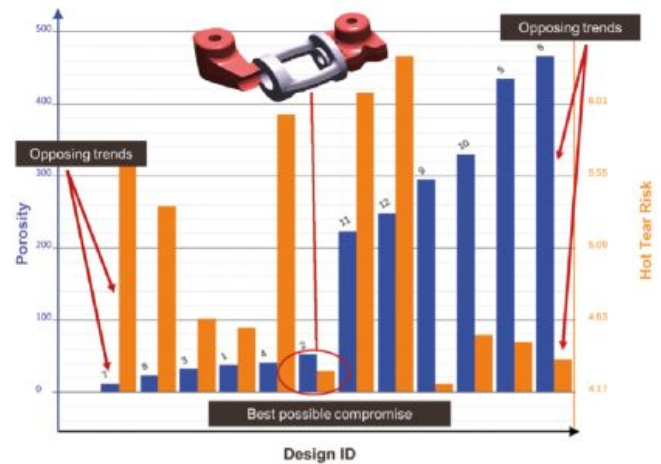
Figure 16. Porosity and related hot tear tendency for all virtual experiments in a bar chart. Design #2 provides the best compromise between the conflicting objectives.
